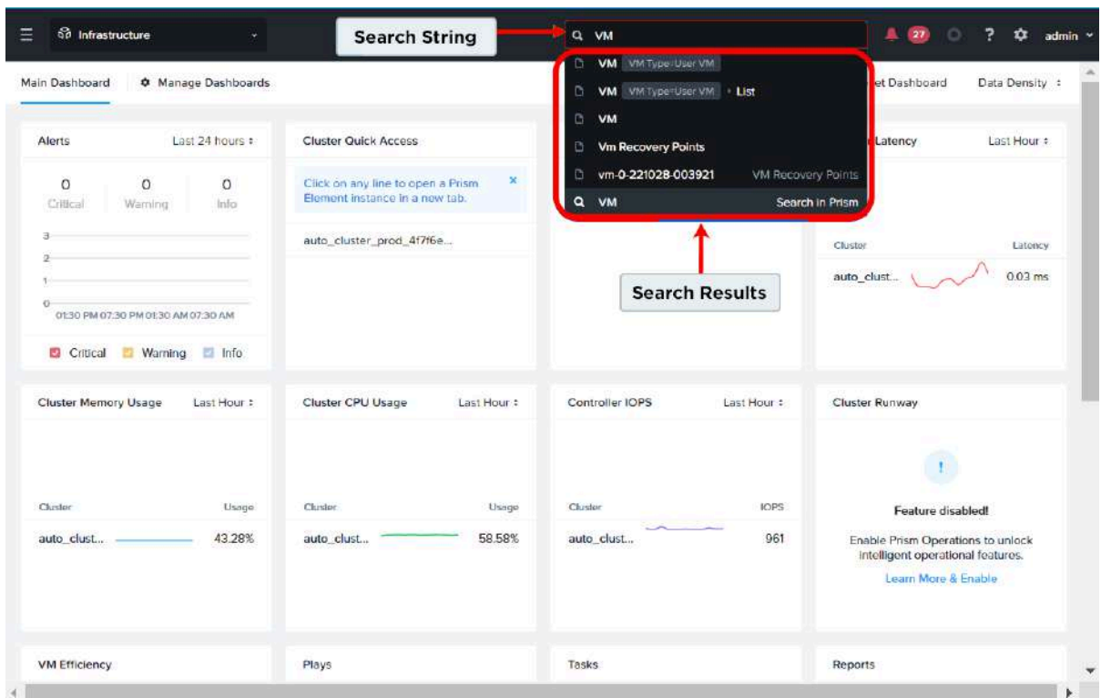
Figure 15: Search Results (for an entity type)
