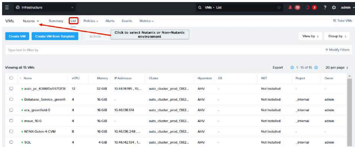
Figure 36: VMs List Tab
