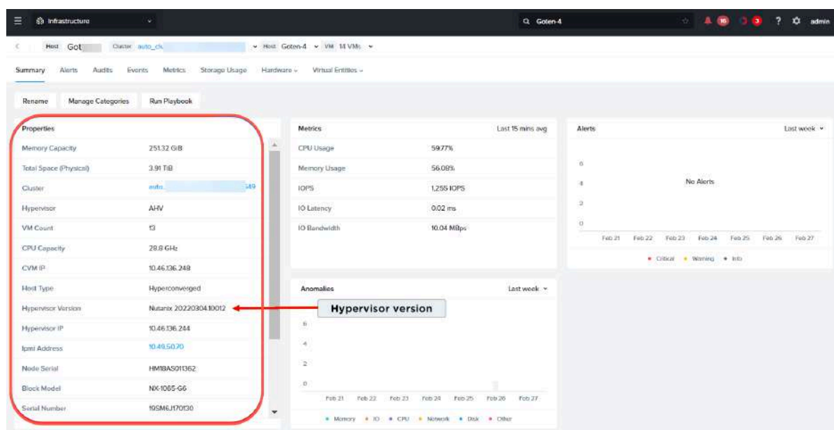
Figure 211: Hypervisor Version in Host Detail View
