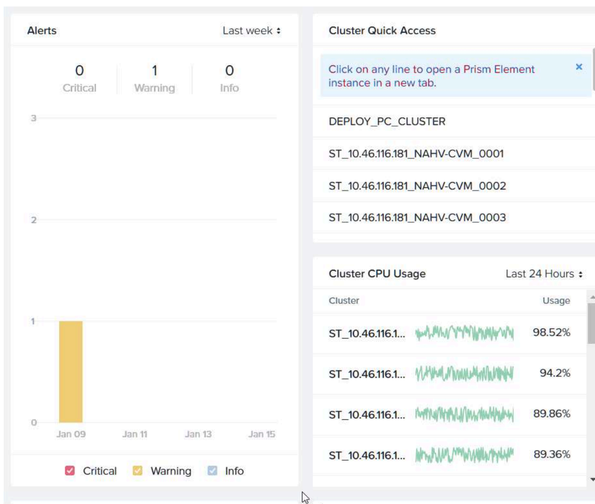
Figure 33: Widget Resize to Twice the Default Length
