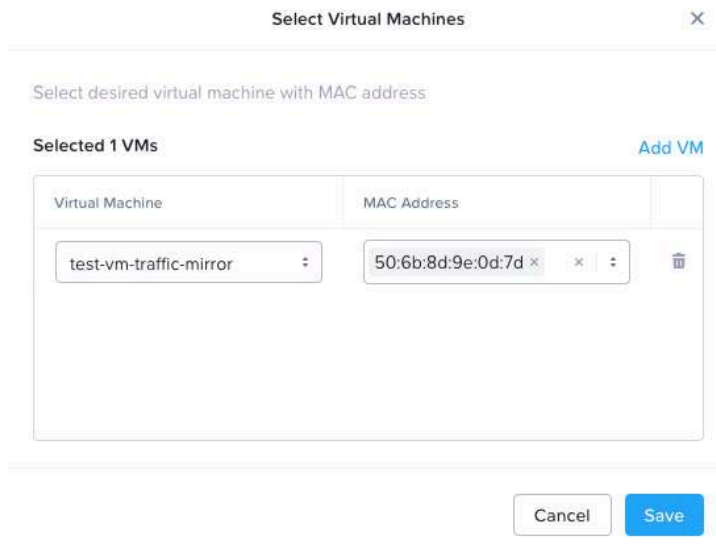
Figure 158: Virtual Machine - Destination
