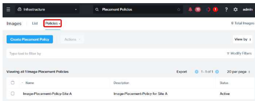
Figure 180: Summary View - All Image Placement Policies
