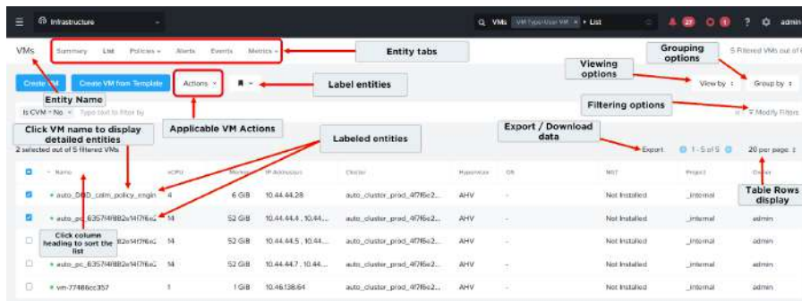
Figure 8: Entity Layout (example)
