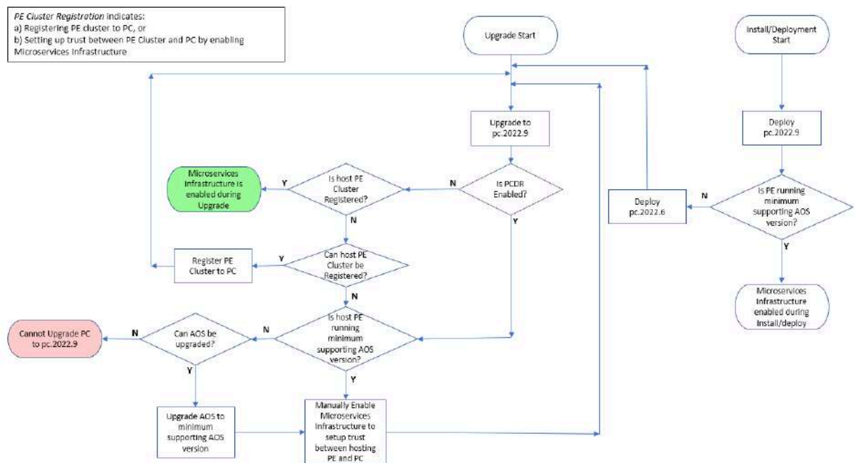
Figure 208: Upgrade/Install Minimum Supporting Prism Central - Process
