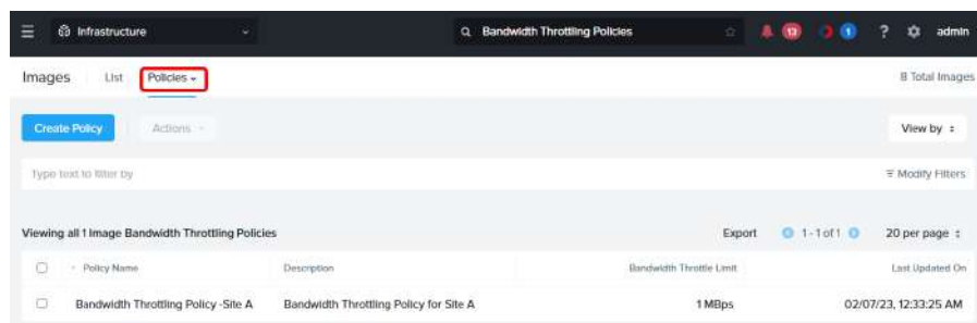
Figure 183: Bandwidth Throttling Policies
