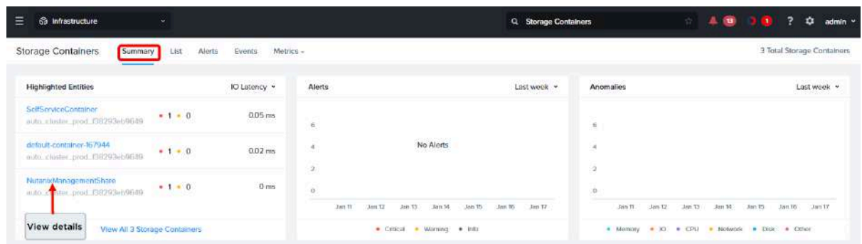
Figure 113: Summary Page - All Storage Containers
