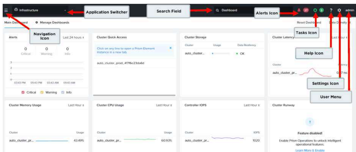
Figure 5: Prism Central Landing Page
